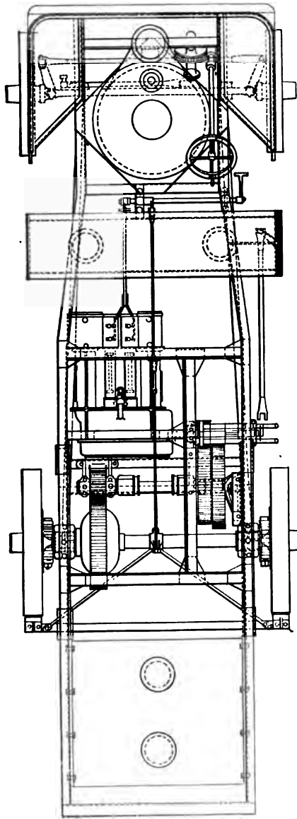
FIG. 73.—Plan of Body and Underframe of Thorncroft Long Frame Lorry. The dotted lines between the axles indicate the reaches which constitute the underframe.
